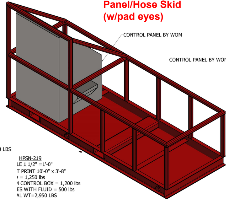
Panel/Hose Skid
