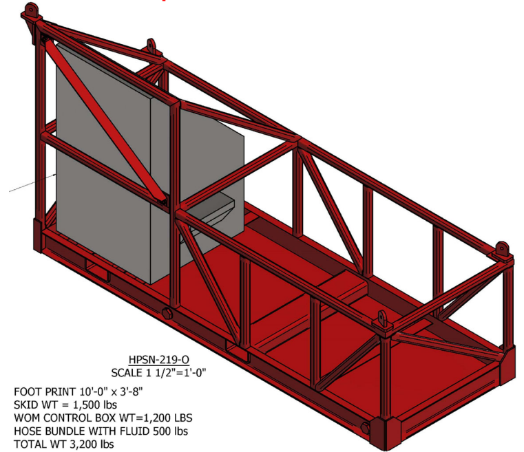
Panel/Hose Skid (w/pad eyes)
